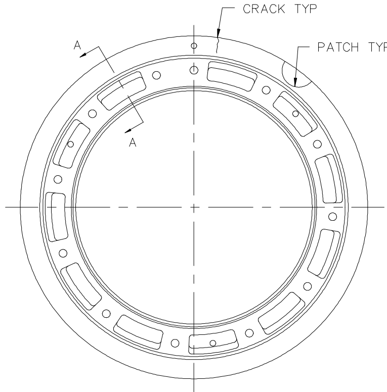
TURBINE NOZZLE
